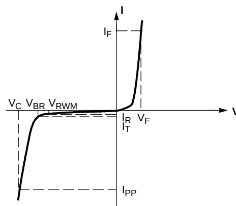
Uni-Directional TVS
