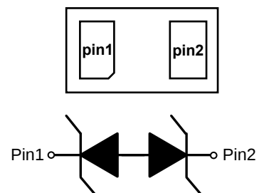
Circuit Diagram
